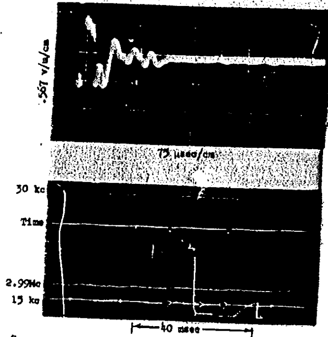
Fig. 3.79 Narrow-band responses Shot No. 7 1000 km from ground zero
